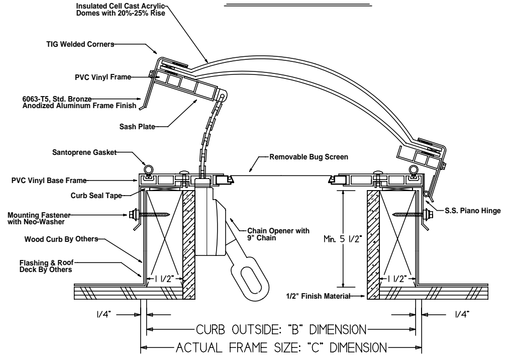
(A) SKYLIGHT CROSS SECTION
